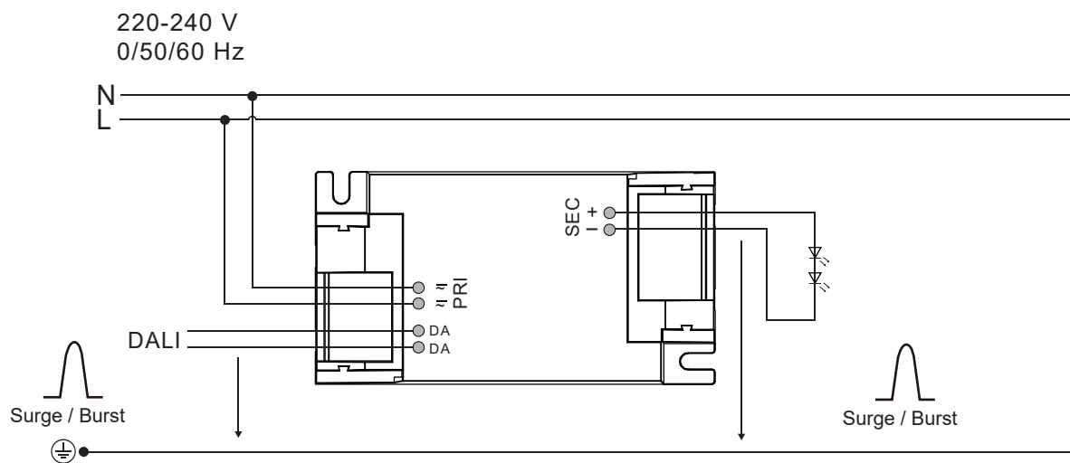
Figure: Voltage peaks for LED driver without earthing (Above) and with earthing (Below)
