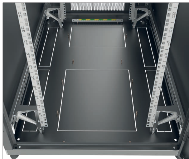
View on the bottom plate
