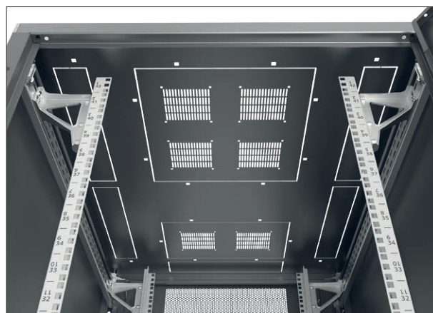
View on the top plate
