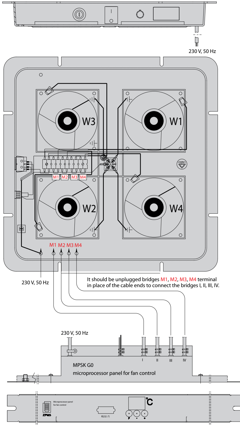
Diagram illustrating the connections of PWD-4W roof fan panel with the MPSK G0 microprocessor panel for fan control
