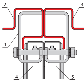
Baying cabinets with side panels
