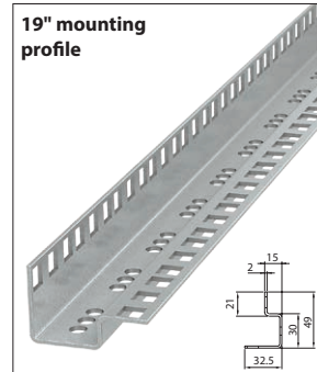
19" middle mounting profile
