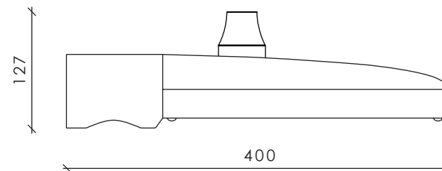
Dimensions with RF antenna
