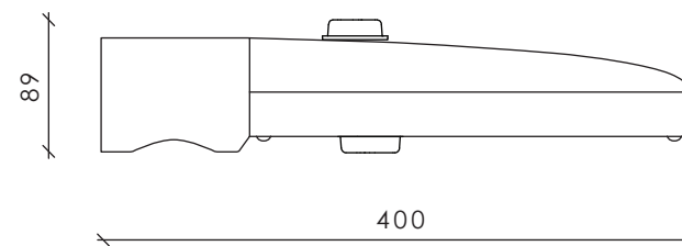
Dimensions with 2 Zhaga connectors
