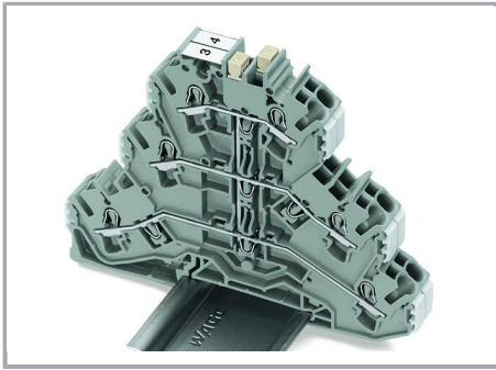
Commoning three levels via triple-deck vertical jumper (2002-493).
