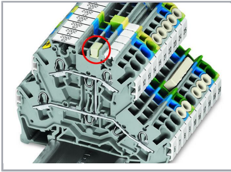
Commoning two levels via double-deck vertical jumper (2002-492).
