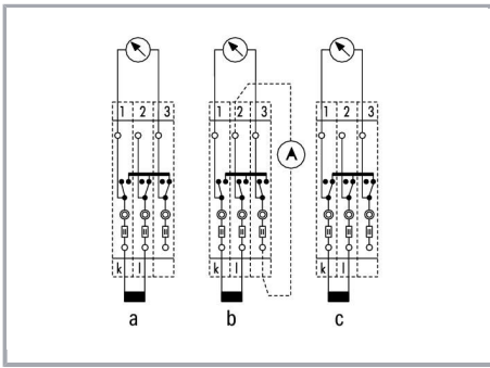
Current transformer circuit with transverse switching terminal blocks
