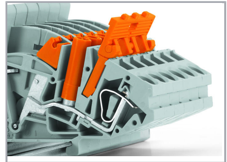
Jumper with raised safety lid
