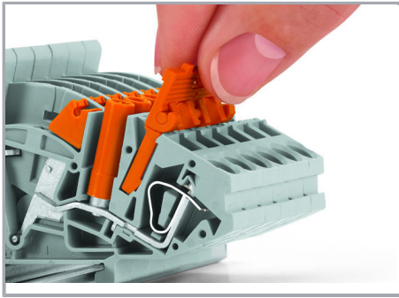
Removing a jumper via safety lid.
