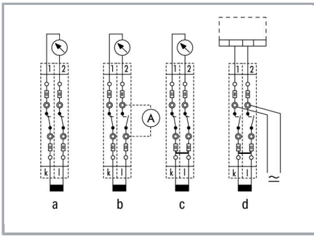
Current transformer circuit with longitudinal switching disconnect terminal blocks
