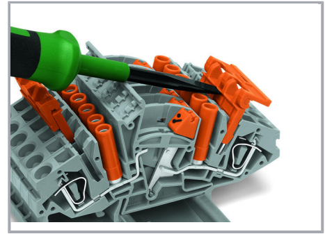
Jumper with safety lid:
