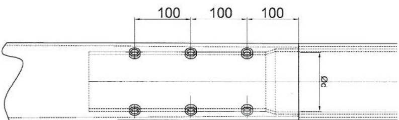
DETAIL OF POLE/BACKET FIXATION (DRV)
