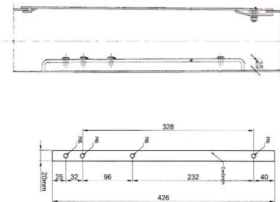
DETAIL OF THE INSIDE OF THE DOOR
